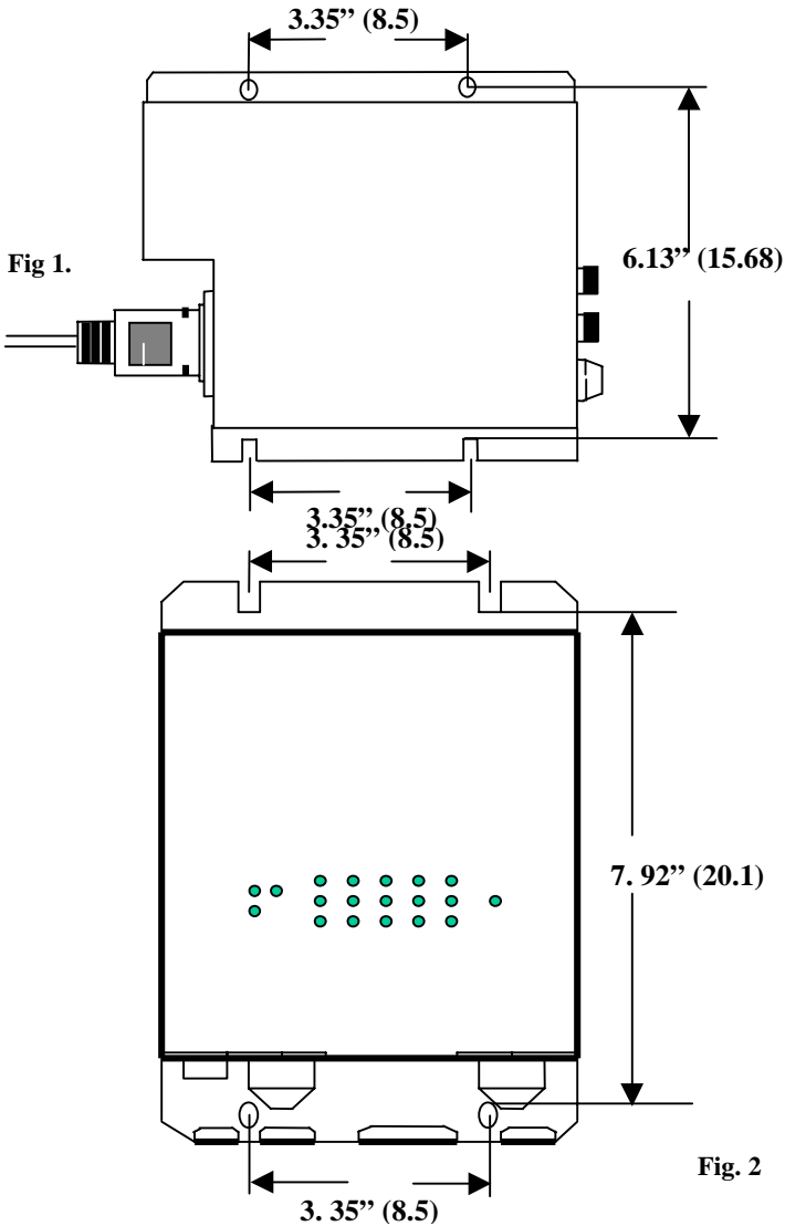
Mounting Hole Dimensions, inches & (cm)
